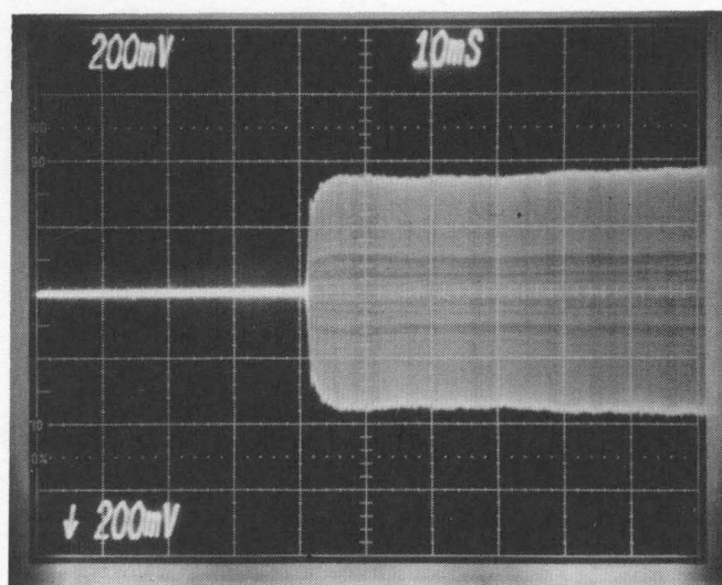
FIGURE 37. HEAD LOAD TIMING
