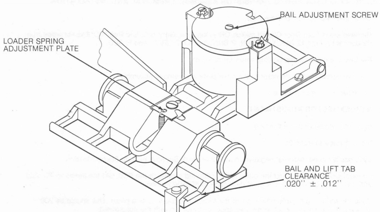
FIGURE 36. HEAD LOAD MECHANISM ADJUSTMENT
